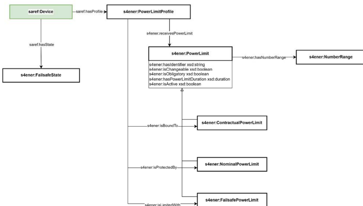
Figure 9 Power Limit Profile
