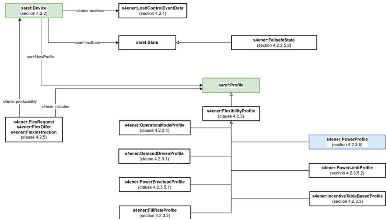
Figure 1: SAREF4ENER overview
