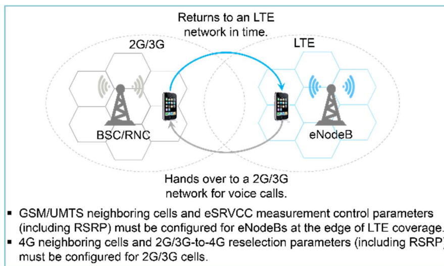
Figure 5-26: Interoperability between VoLTE and 2G and 3G
