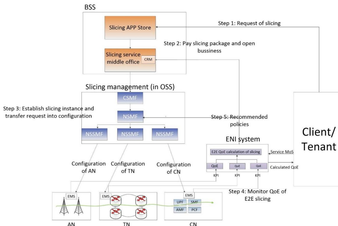
Figure 5-32: Possible deployment scenario of Service experience optimization of E2E slicing involving both BSS and OSS
