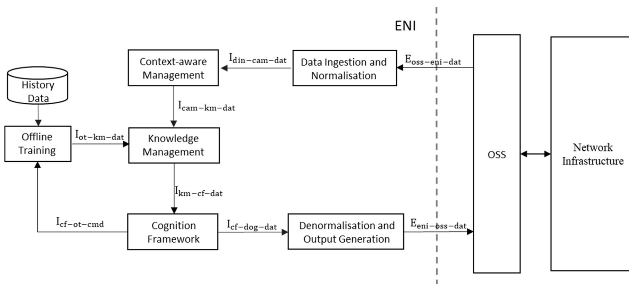
Figure 5-17: Mapping to ENI reference architecture (option one)
