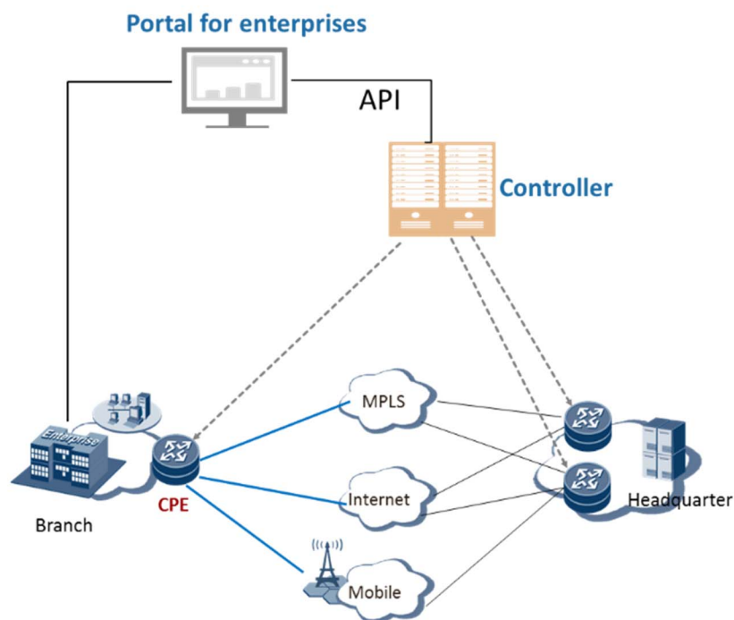
Figure 5-30: Intelligent carrier managed SD-WAN service
