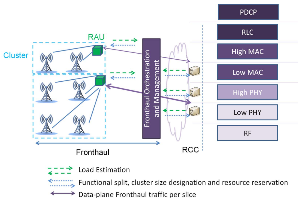
Figure 5-10: Concept of the proposed Fronthaul use case
