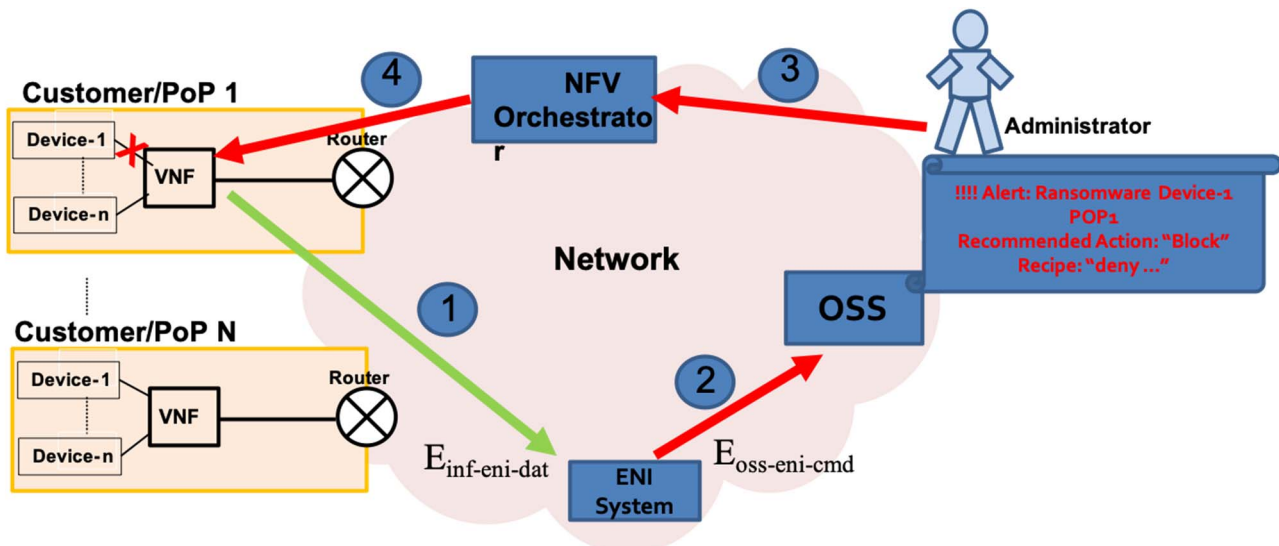
Figure 5-39: Use case to limit profit in cyber-attacks using NFV and ENI system
