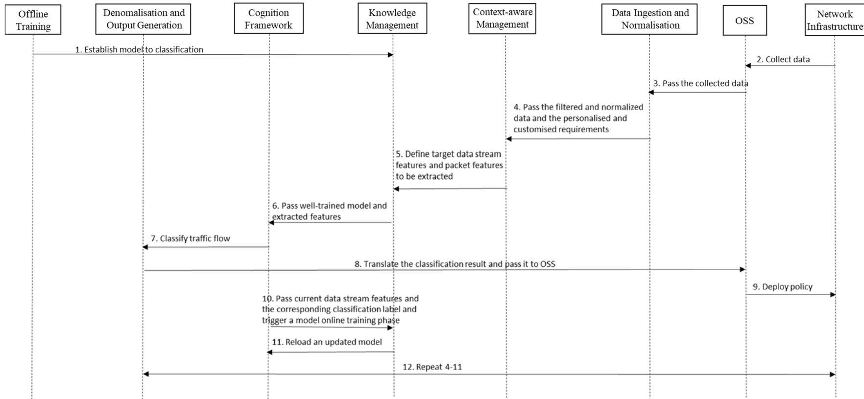
Figure 5-20: Scenario of AI enabled network traffic classification (option two)
