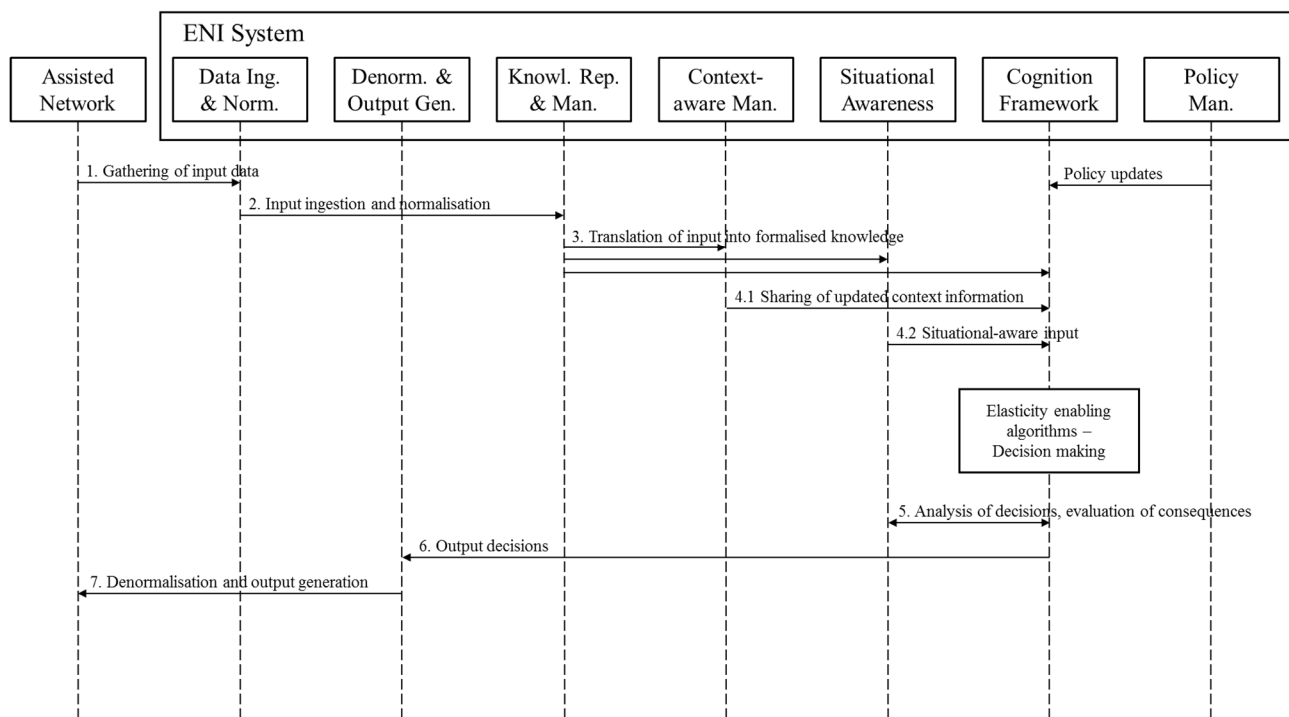
Figure 5-12: Example Flow of information among the ENI System's functional blocks and the Assisted System
