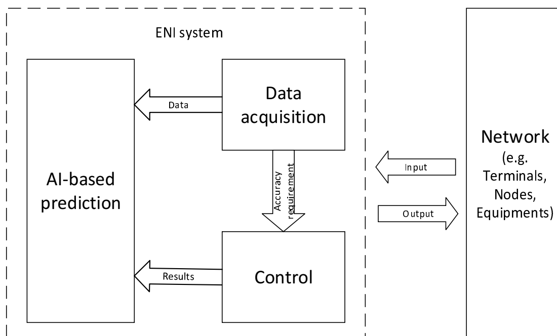
Figure 5-23: Intelligent time synchronization of network
