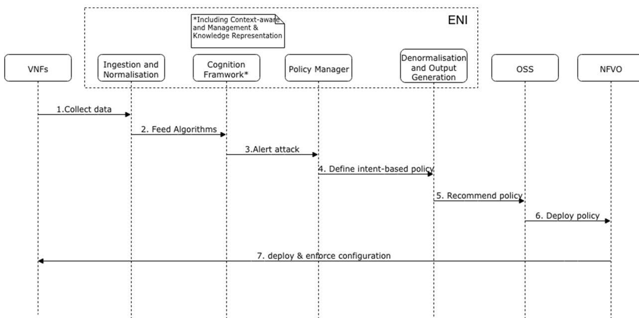
Figure 5-40: Flow of information among the ENI System's functional blocks and the Assisted System
