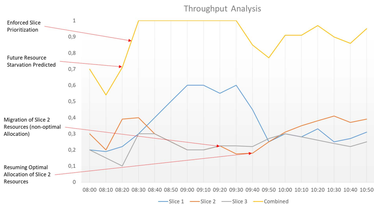
Figure 5-36: High priority Network Slice Assurance
