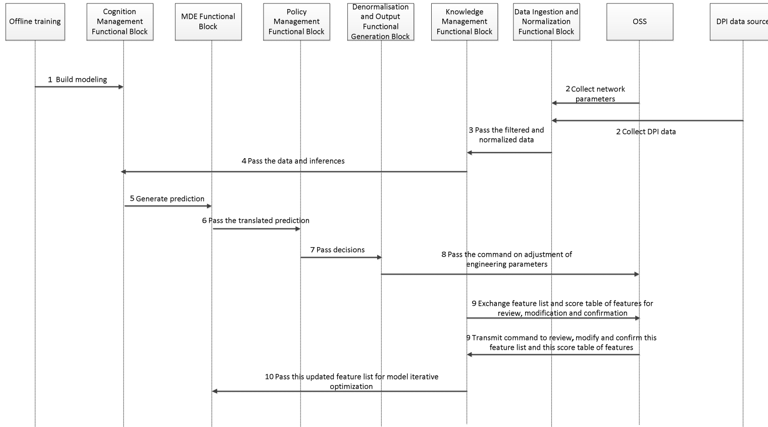
Figure 5-15: Flow of information for Application Characteristic based Network Operation
