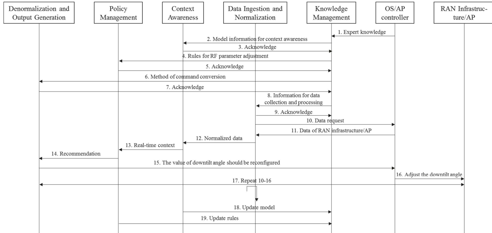
Figure 5-9: Procedure for coverage and capacity optimization
