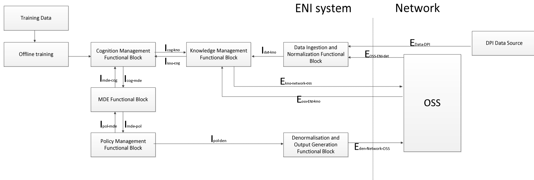
Figure 5-14: Mapping to ENI reference architecture for Application Characteristic based Network Operation
