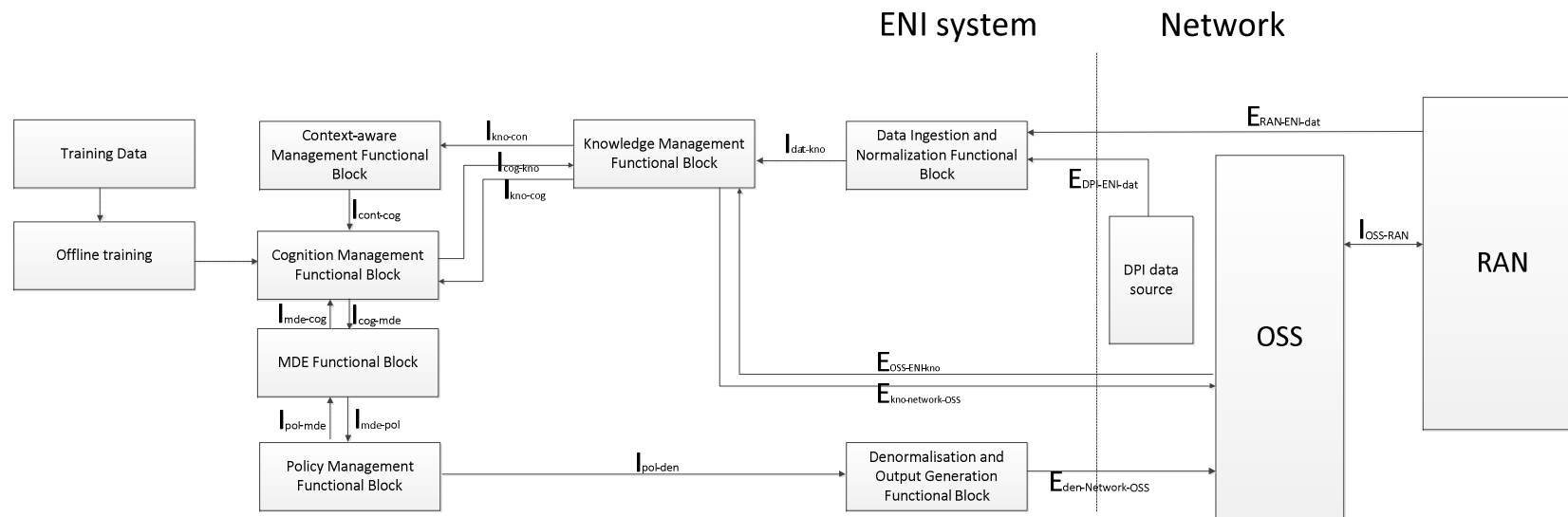
Figure 5-27: Mapping to ENI reference architecture for Context-aware VoLTE Service Experience
