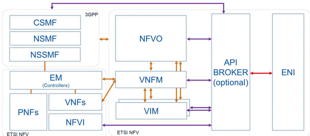
Figure 5-11: An architectural design including ETSI NFV MANO, 3GPP management functions, and ENI engine
