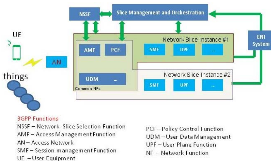
Figure 5-29: Example of a network slicing management and orchestration scenario
