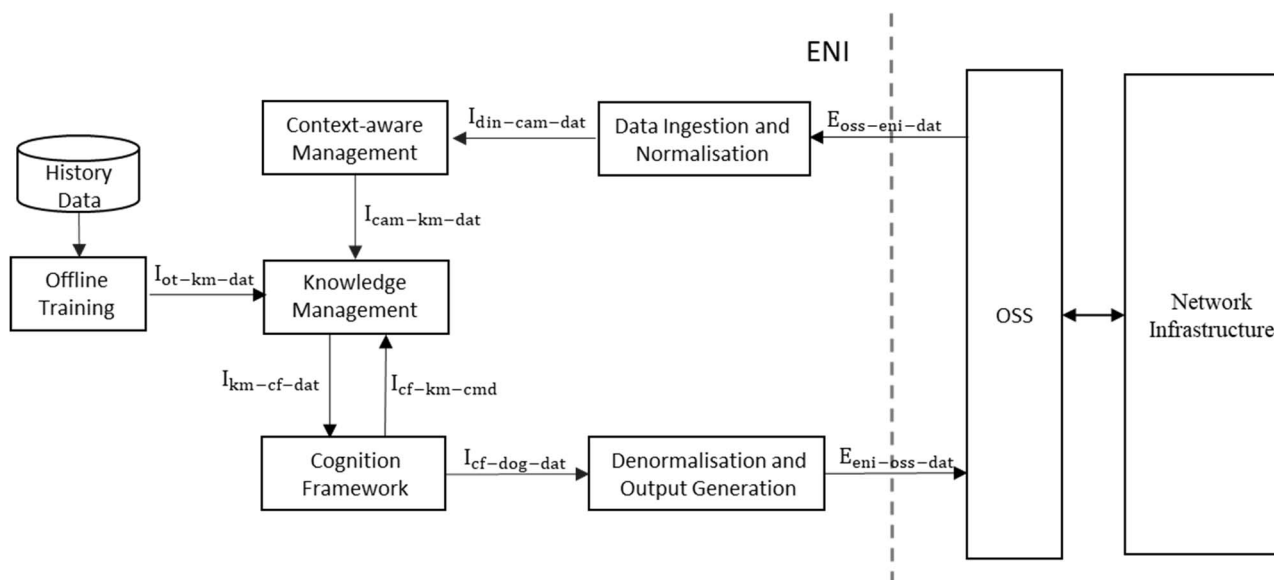
Figure 5-18: Mapping to ENI reference architecture (option two)
