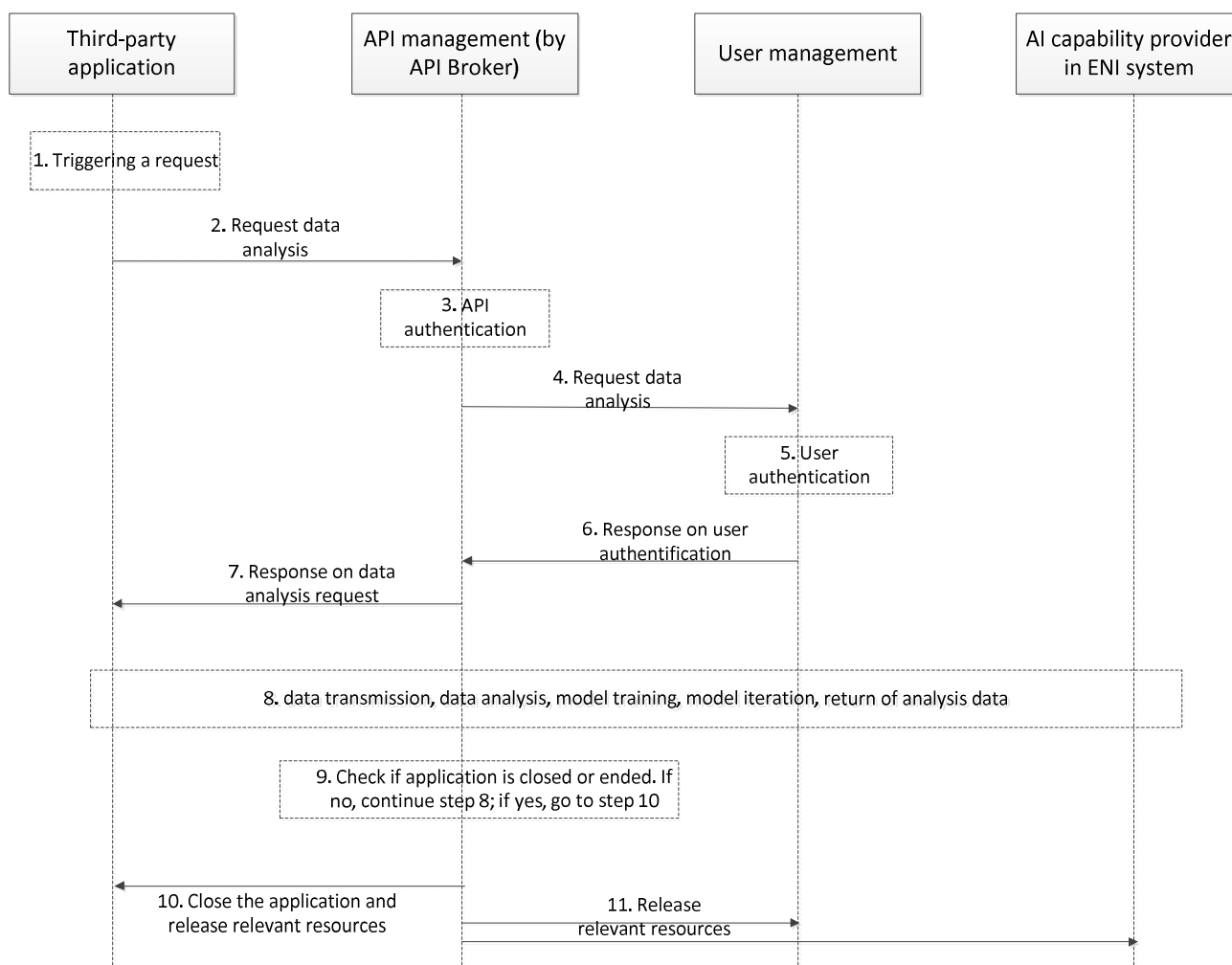
Figure 5-43: Flow of information for "exposure of AI capability from ENI system"
