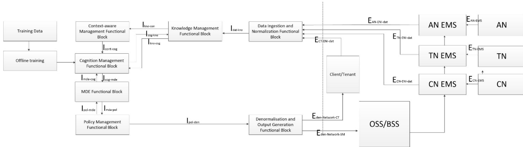
Figure 5-33: Mapping to ENI reference architecture for service experience optimization of E2E slicing considering both BSS and OSS
