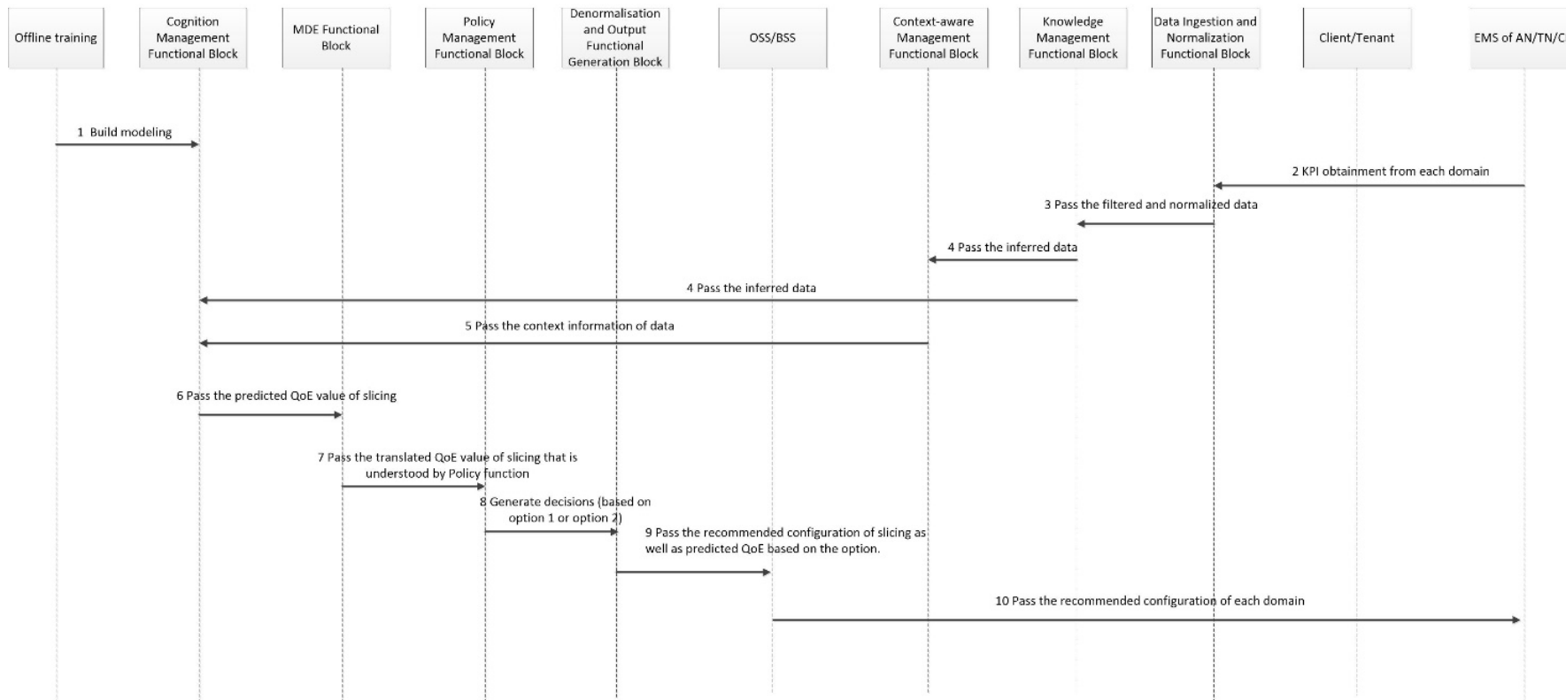
Figure 5-34: Flow of information for "service experience optimization of E2E slicing involving both BSS and OSS"
