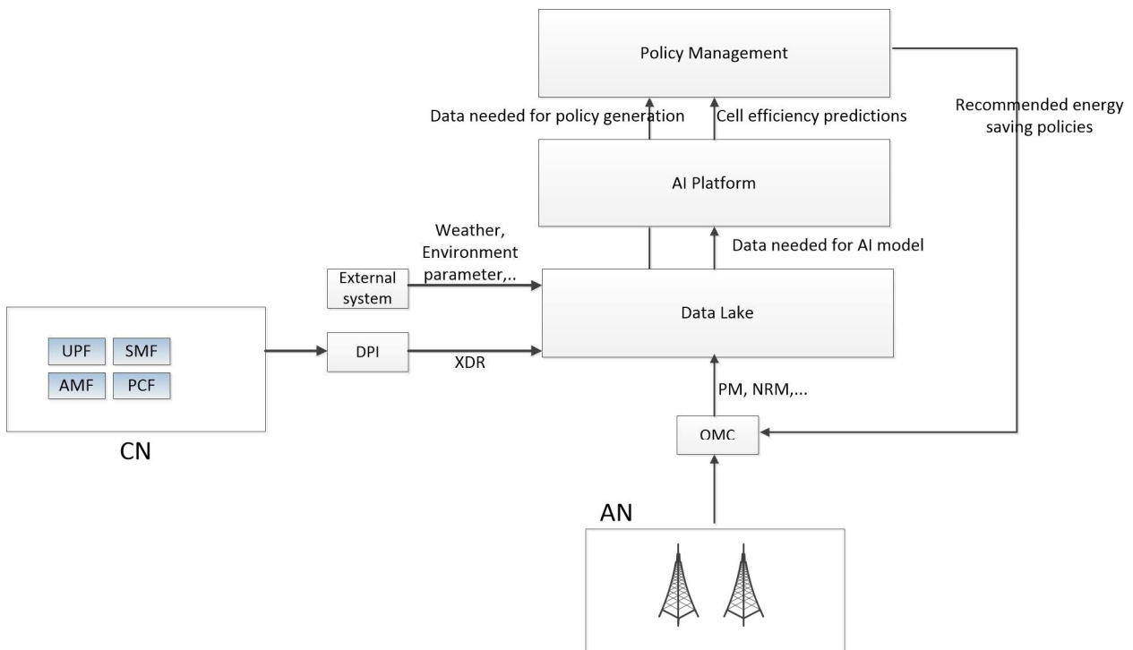
Figure 5-41: Energy saving for radio network
