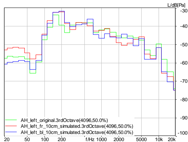
Figure 11: Original (green curve) and simulated power density spectra measured at the left ear of the artificial head
