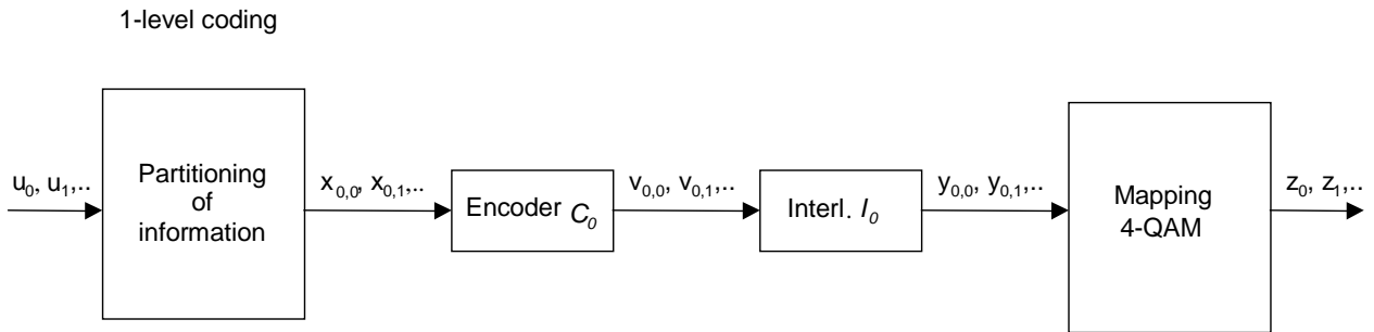
Figure 24: Multilevel coding with 1 level
