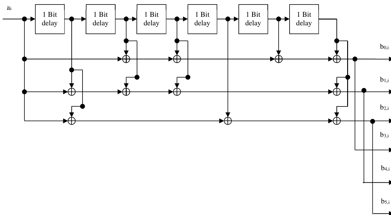
Figure 25: Convolutional encoder
