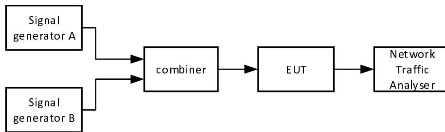
Figure 13: Test setup for co-channel rejection
